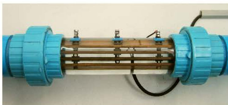
Ionizer cell with copper plates
